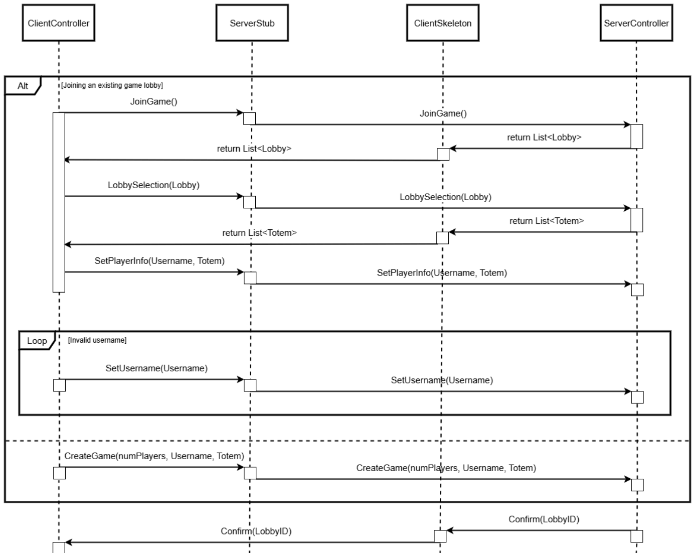
Game access RMI sequence diagram
